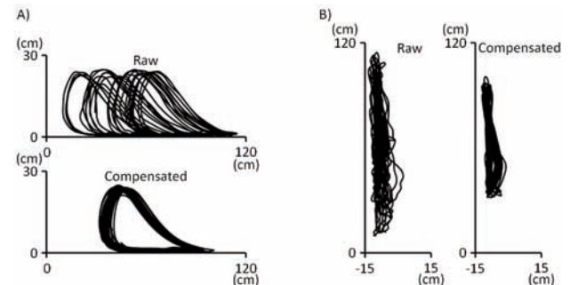
Figure 3. Raw and compensated marker trajectories attached to the right lateral malleolus. A) View from the sagittal plane. B) View from the horizontal plane.
